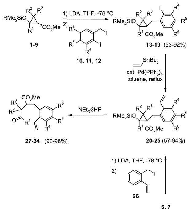
Scheme 2. (For R, R 1 –R 6 see Table 1.).
