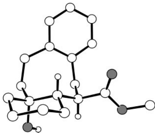
Figure 1. Benzocyclooctanol derivative 47 (only selected hydrogen atoms are depicted).
